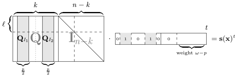
Fig. 1. Collision Decoding by Stern - \mathbf{H}\mathbf{e}^t = \mathbf{s}(\mathbf{x})^t . The error vector \mathbf{e} contains two blocks each of \frac{p}{2} 1's in its upper half corresponding to the columns of \mathbf{Q}_{I_1} and \mathbf{Q}_{I_2} . Since \mathbf{Q}_{I_1} and \mathbf{Q}_{I_2} sum up to \mathbf{s}(\mathbf{x}) on the rows defined by [\ell] we have to fix a corresponding zero-block in coordinates \{k + 1, \dots, k + \ell\} of \mathbf{e} . The remaining (\omega - p) 1's are then distributed over the remaining coordinates \{k + \ell + 1, \dots, n\} of \mathbf{e} .
